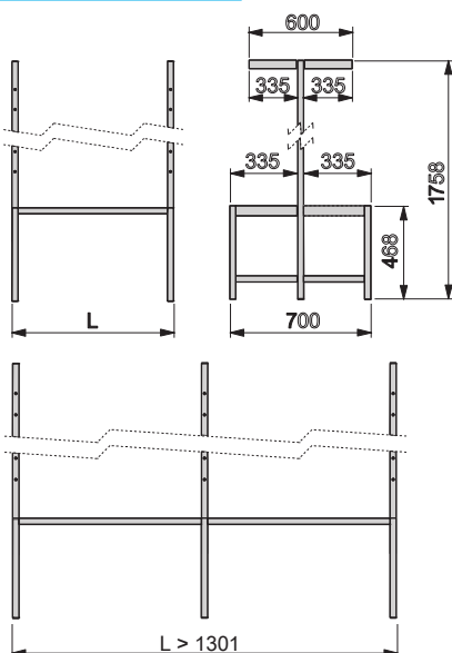
Double bench with hook and top shelf
